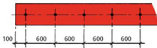
REF. '1' CENTRE LINE
