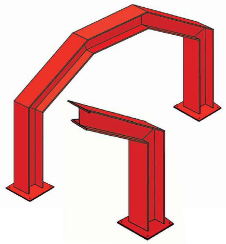
REF. '1' THROUGH WEB
