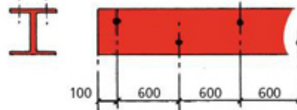
REF. '2' THROUGH TOP FLANGE
