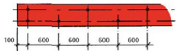
REF. '2' STAGGERED
