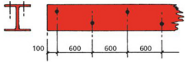
REF. '2' THROUGH TOP FLANGE
